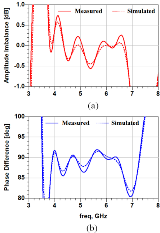
Fig. 6. (a) Simulated and measured amplitude imbalance of the proposed HMSIW quadrature power divider. (b) Simulated and measured phase difference.
